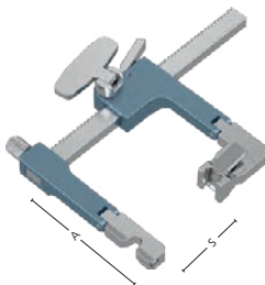
BB-Retraktor Offset BB-Retractor offset
